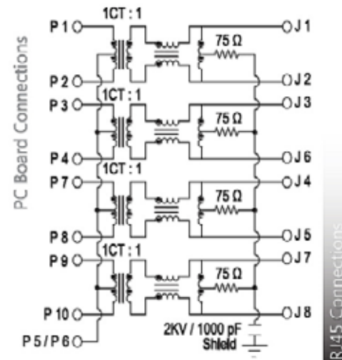
SCHEMATIC NO. G6
