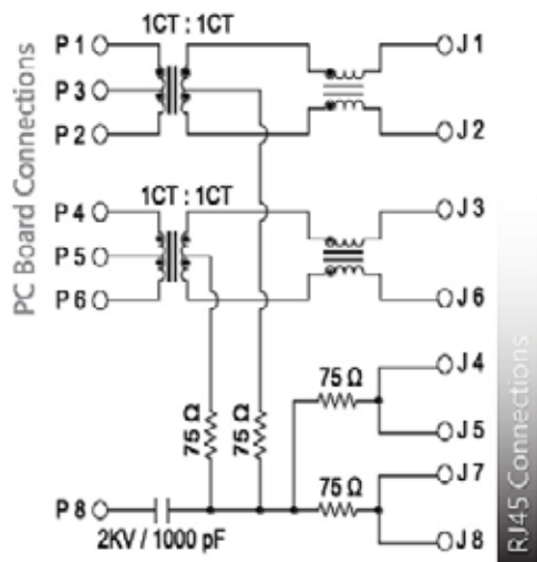
SCHEMATIC NO. 51
