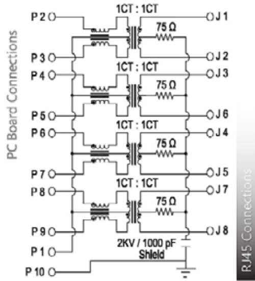
SCHEMATIC NO. G9
