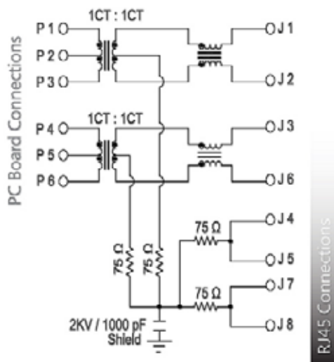
SCHEMATIC NO. 77
