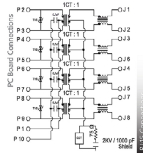
SCHEMATIC NO. J9 (SURGE)
