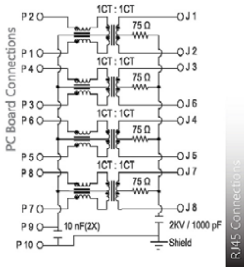
SCHEMATIC NO. H4
