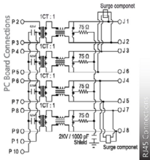
SCHEMATIC NO. J1 (SURGE)
