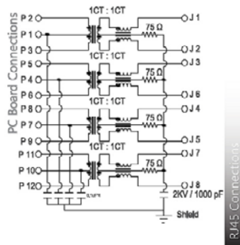
SCHEMATIC NO. J3
