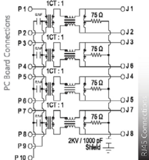
SCHEMATIC NO. G3
