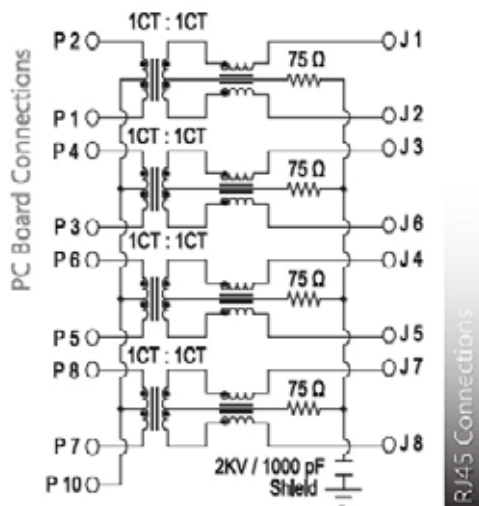
SCHEMATIC NO. G1
