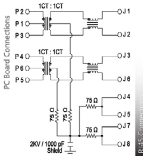
SCHEMATIC NO. 67
