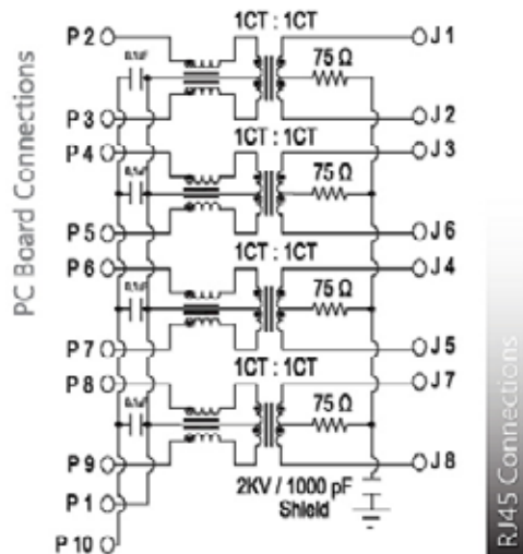
SCHEMATIC NO. G4
