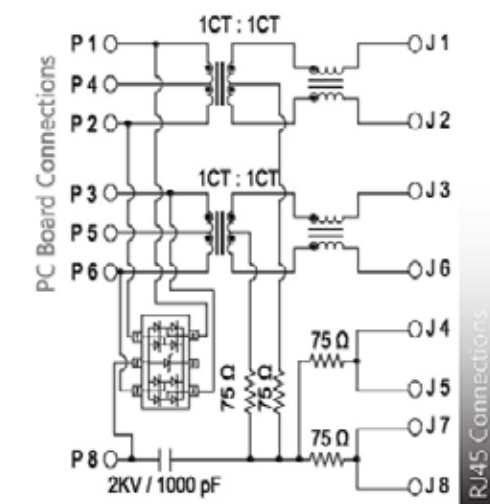
SCHEMATIC NO. 62 (SURGE)
