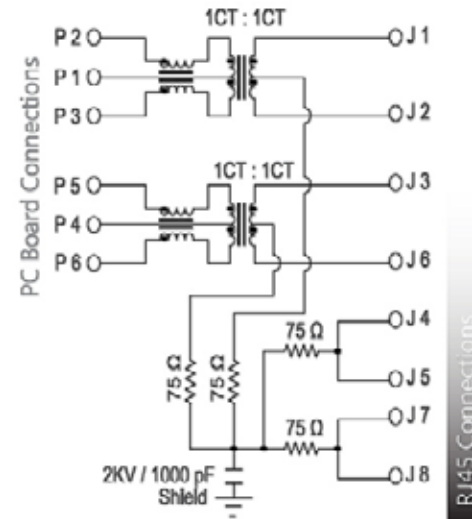
SCHEMATIC NO. 76
