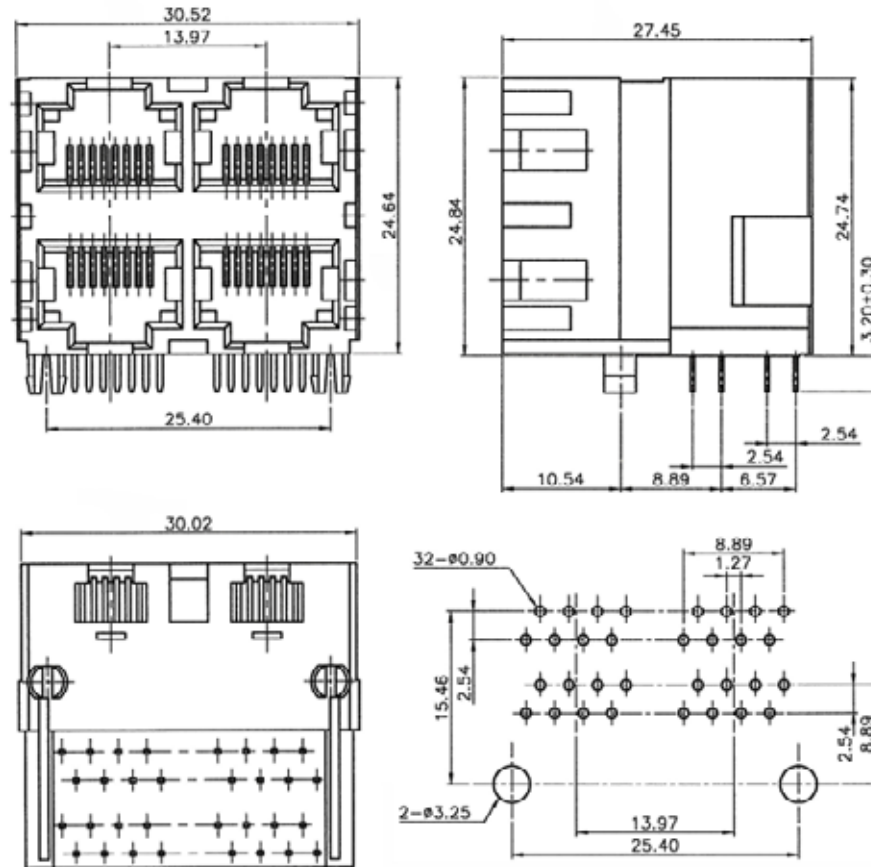
Recommended P.C.Board Layout (TOP VIEW)
