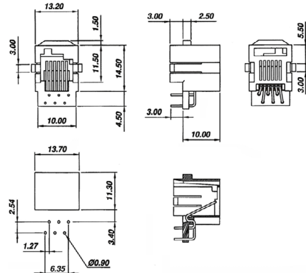
Recommended P.C.Board Layout (BOTTOM VIEW)
