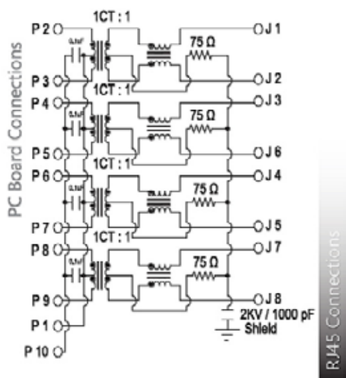
SCHEMATIC NO. H0
