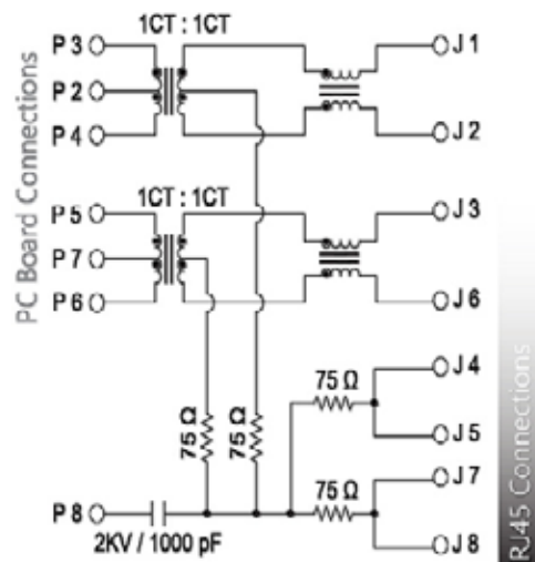
SCHEMATIC NO. 52
