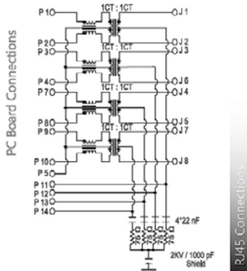
SCHEMATIC NO. J2 (POE)
