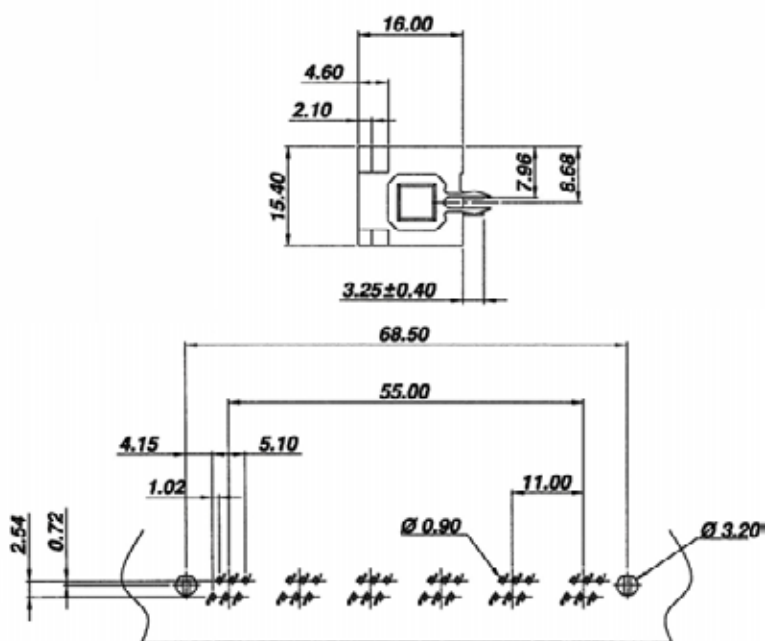
Recommended P.C.Board Layout (TOP VIEW)
