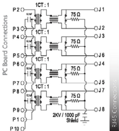
SCHEMATIC NO. G8
