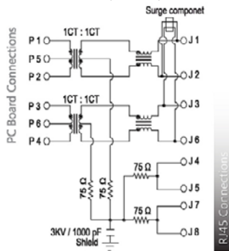
SCHEMATIC NO. 73 (SURGE)
