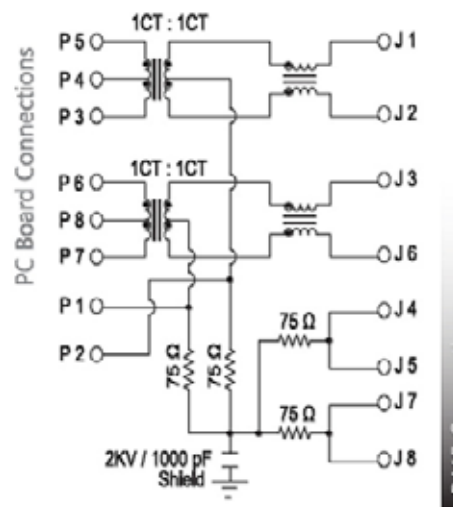
SCHEMATIC NO. 68
