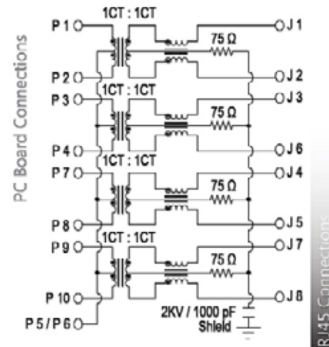
SCHEMATIC NO. G7
