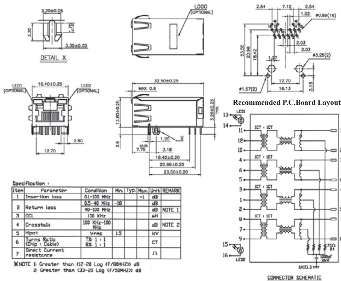
TRANSFORMER TYPE T1
