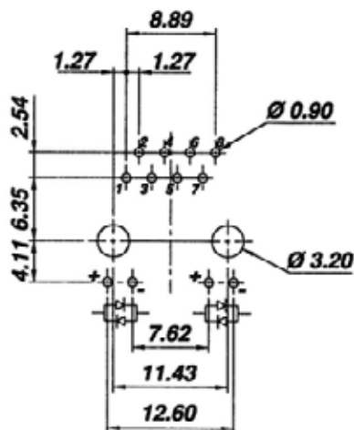
Recommended P.C.Board Layout (TOP VIEW)
