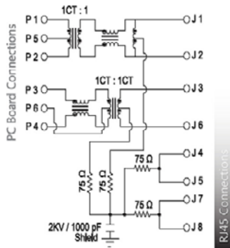
SCHEMATIC NO. 58
