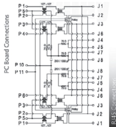
SCHEMATIC NO. 75
