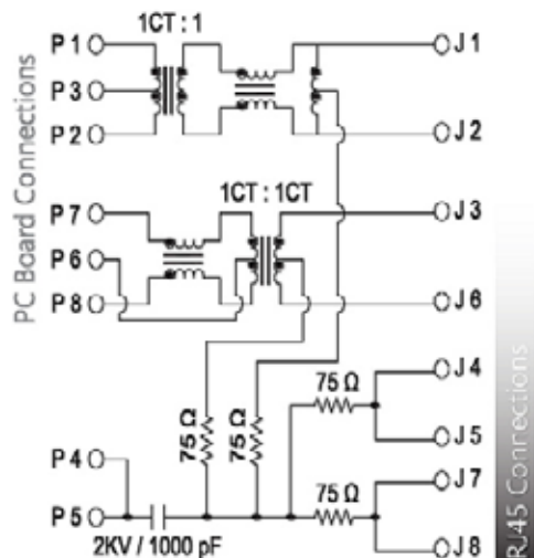
SCHEMATIC NO. 56
