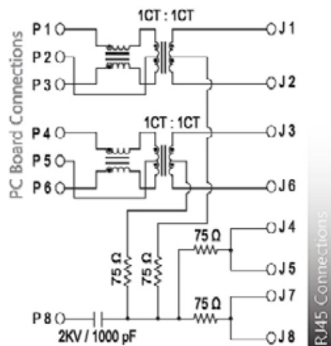
SCHEMATIC NO. 55
