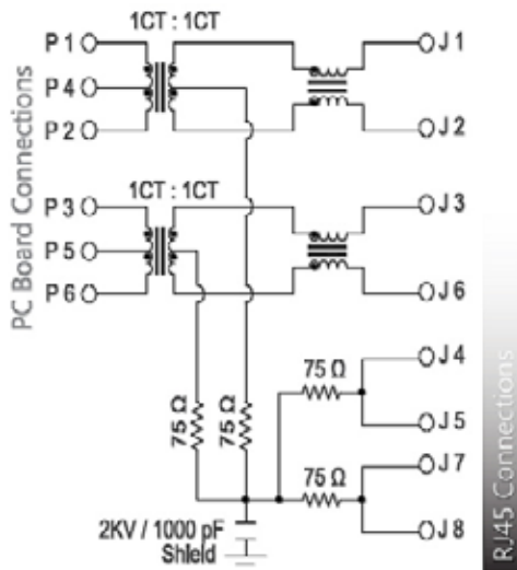
SCHEMATIC NO. 79
