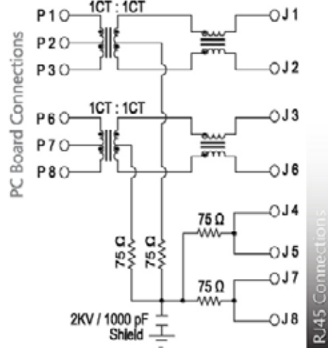
SCHEMATIC NO. 70
