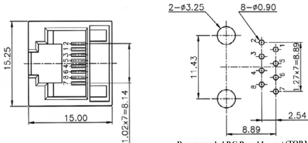
Recommended P.C.Board Layout (TOP VIEW)
