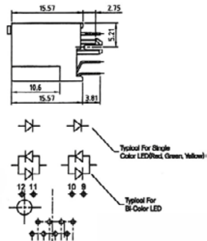
LED SCHEMATIC
