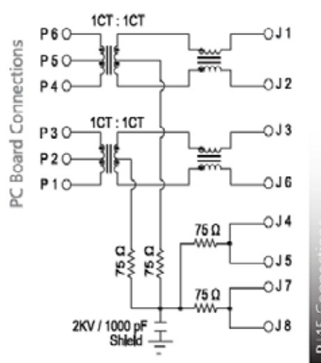
SCHEMATIC NO. 66 (POE)
