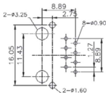
Recommended P.C.Board Layout (TOP VIEW)
