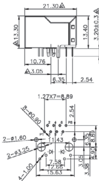
Recommended P.C.Board Layout
