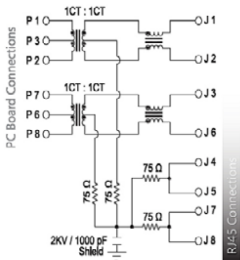
SCHEMATIC NO. 63
