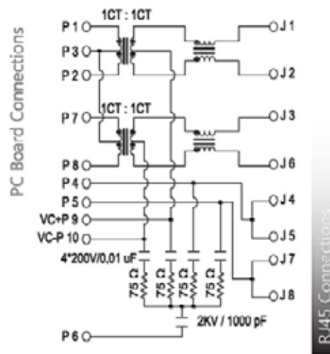
SCHEMATIC NO. 64 (POE)
