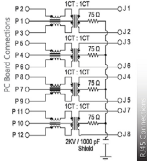
SCHEMATIC NO. G5
