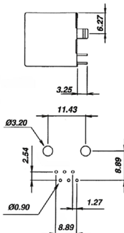
Recommended P.C.Board Layout (TOP VIEW)
