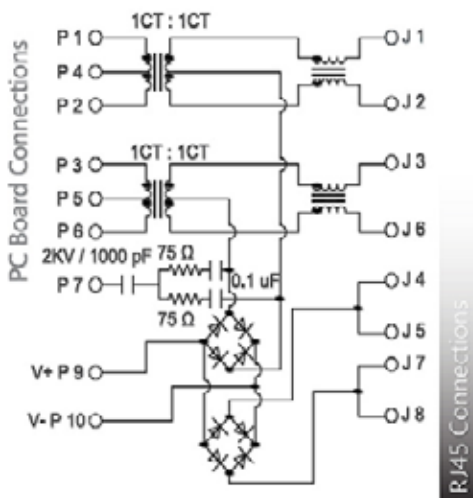
SCHEMATIC NO. 81 (POE)
