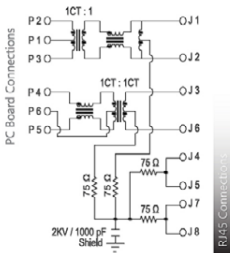
SCHEMATIC NO. 74
