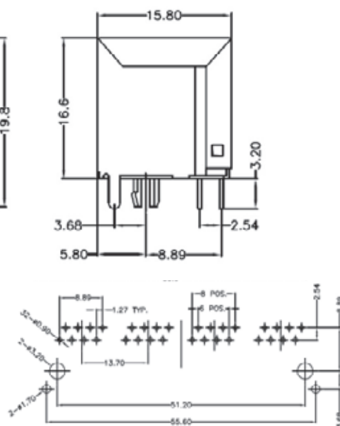
Recommended P.C.Board Layout (TOP VIEW)
