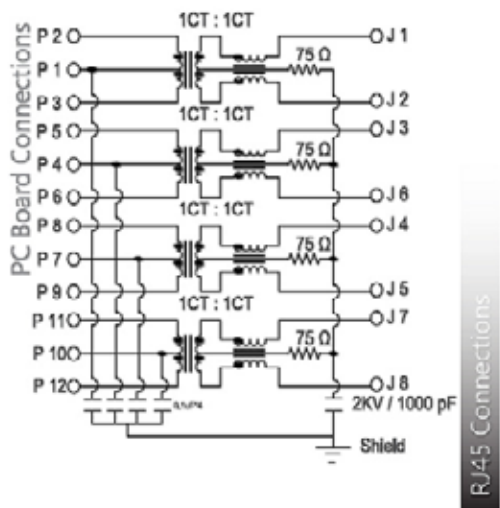
SCHEMATIC NO. J0 (10GB)
