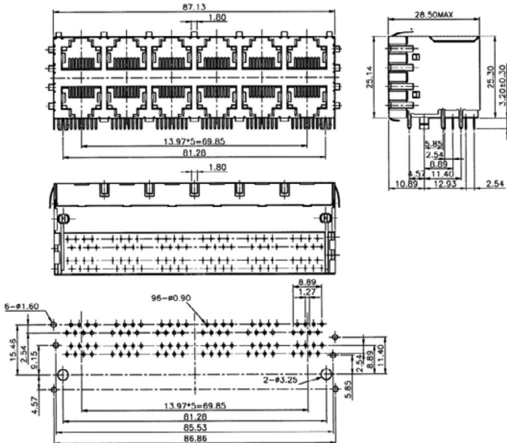
Recommended P.C.Board Layout (TOP VIEW)
